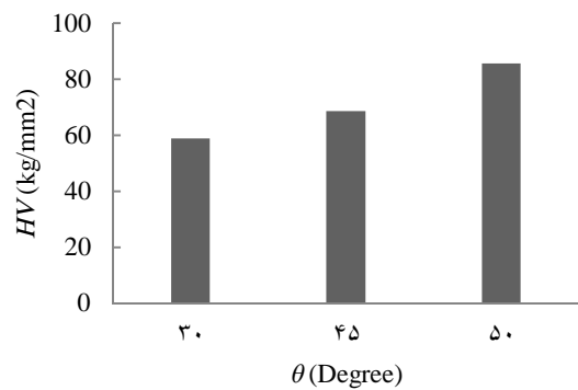
Fig. 16 The effect of groove angle on Vickers hardness of Al 5052 sheet fabricated by one pass of CGP process
