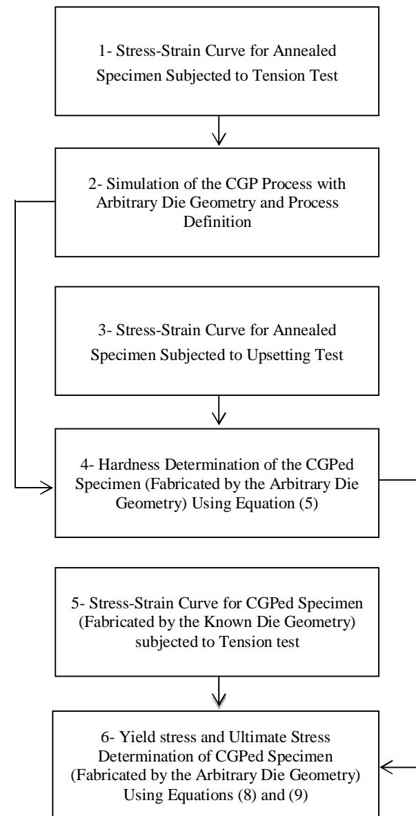
Fig. 7 The algorithm for prediction of die geometry effects on strength behavior of the sheets fabricated by groove pressing process
