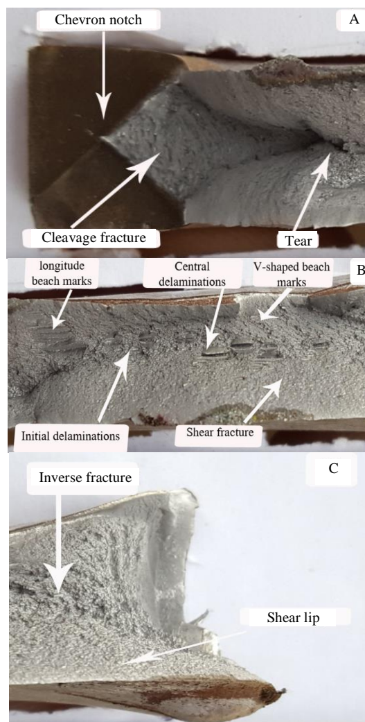
Fig. 12 Fracture surface of left part of DWT specimen with crack growth direction from left to right: (A) first section: initial 23 mm crack growth, (B) second section: 23-63 mm crack growth and (C) third section: 63-79 mm crack growth
