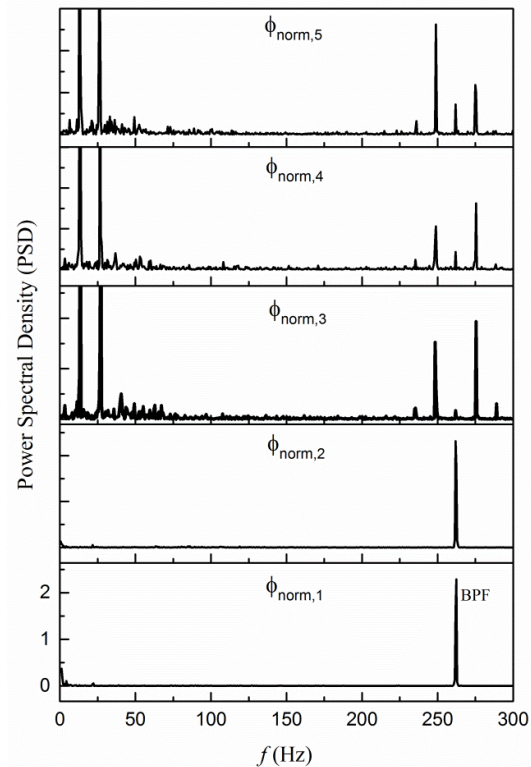
Fig. 5 Velocity spectra in the frequency domain during different operating conditions
