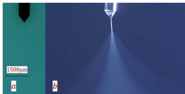
Fig. 13 Cone jet mode, (a): from shadowgraph, (b): from light scattering, Flowrate= 2 ml/h, Voltage= 4.63kV
