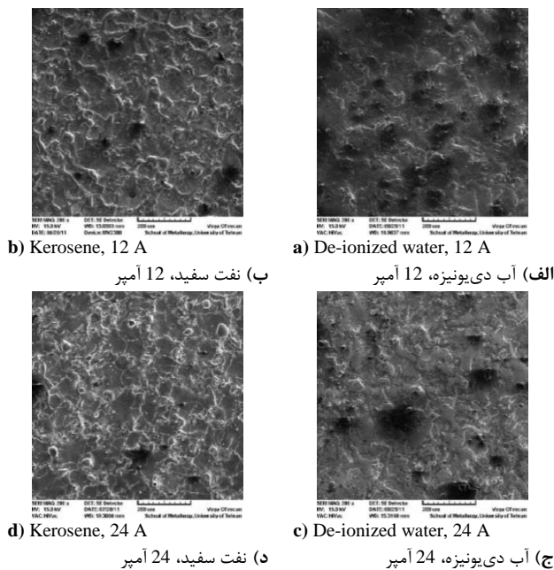
Fig. 5 Machined surface topography by SEM images with 200 X magnification for the 6.4 \mu s pulse on time
