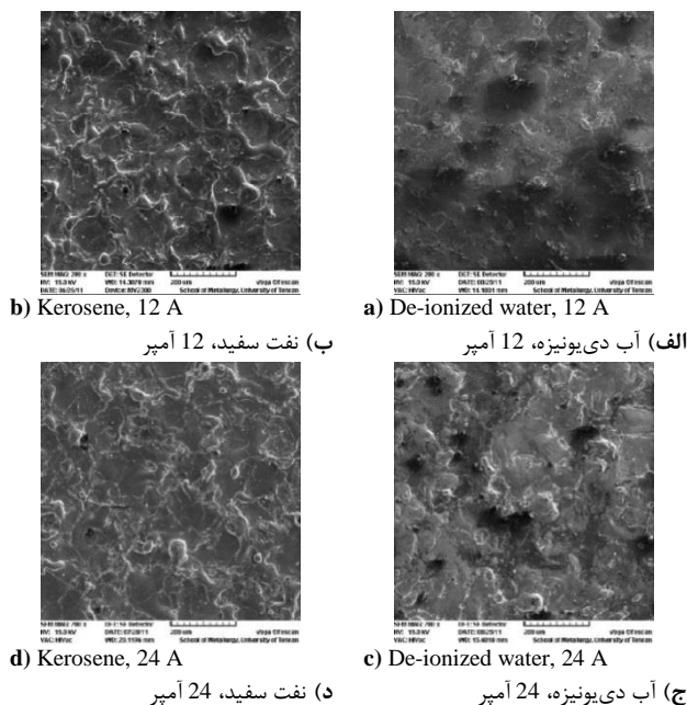
Fig. 6 Machined surface topography by SEM images with 200 X magnification for the 12.8 \mu s pulse on time
