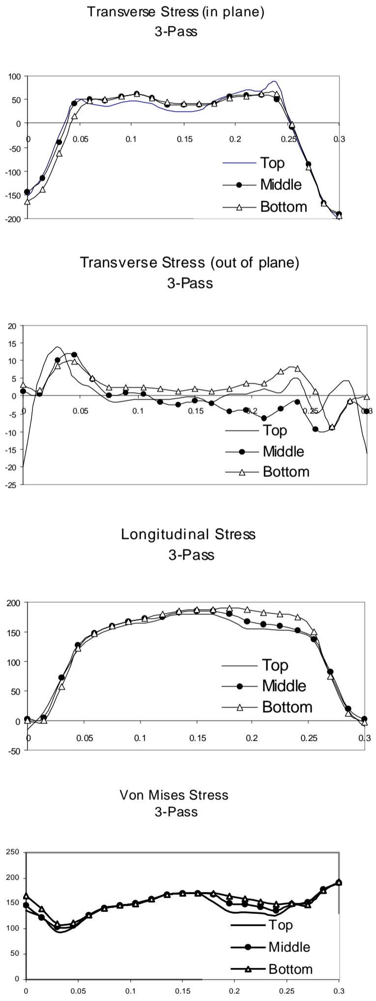
Fig. 6 Variation of different components of residual stresses through the thickness of plates (stresses and distance are measured in Mpa and meter respectively).
