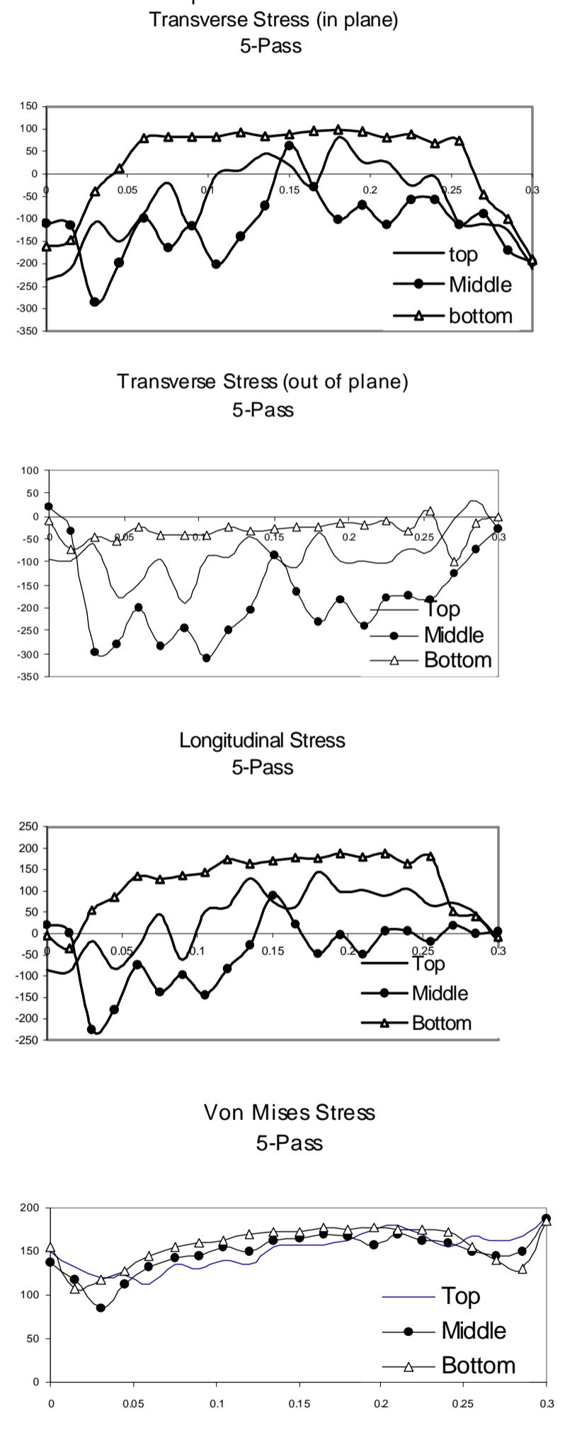
Fig. 6 Variation of different components of residual stresses through the thickness of plates (stresses and distance are measured in Mpa and meter respectively).
