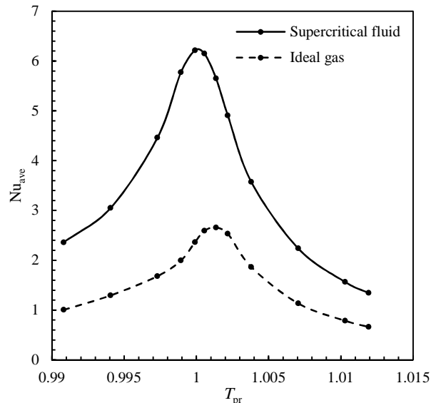
Fig.11 Nusselt numbers for a tube of 0.4mm diameter and temperature difference of 1 degree at 8MPa
