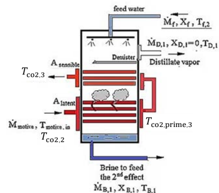
Fig. 4 schematic diagram of first effect with hot supercritical CO_2 as sensible heat source
