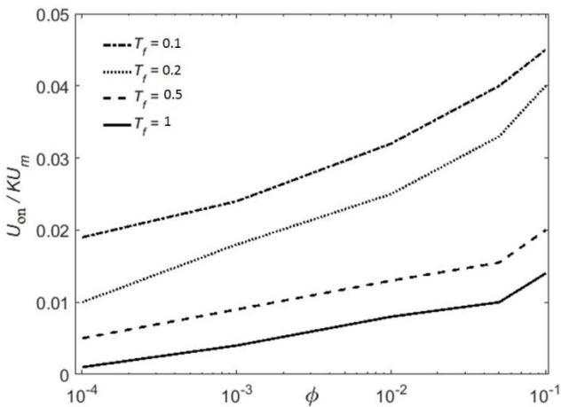
Fig. 13 Preferred regions of u_{on} versus \phi for different values of T_f = 0.1, 0.2, 0.5, 1 in detumbling mode ( k_d = 1 )
