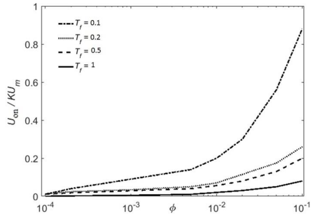
Fig. 10 Preferred regions of u_{on} versus \phi for different values of T_f = 0.1, 0.2, 0.5, 1 without reference input ( k_d = 1 )
