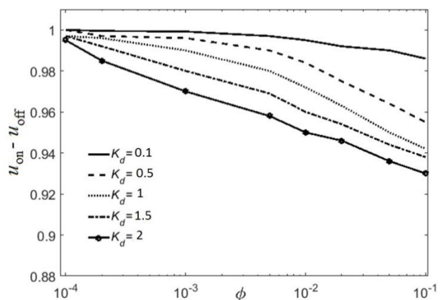
Fig. 12 Preferred regions of h versus \phi for different values of k_d = 0.1, 0.5, 1, 1.5, 2 without reference input ( T_f = 0.5 )
