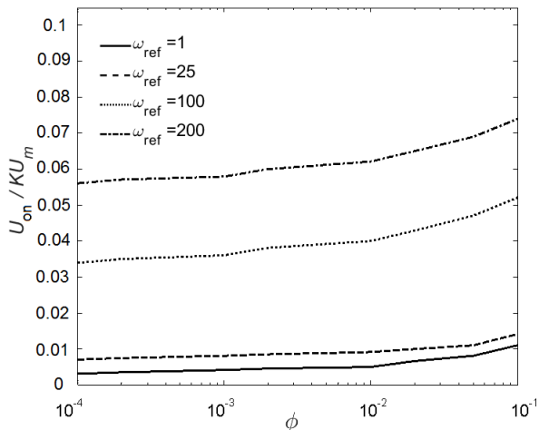
Fig. 16 Preferred regions of u_{on} versus \phi in tumbling mode for different values of \omega_{ref}=1, 25, 100, 200 ( k_d = 0.2, T_f = 0.5 )
