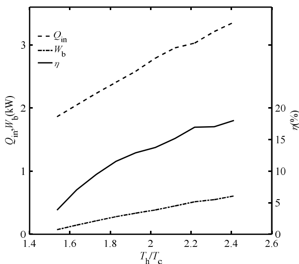
Fig. 18 Heat consumption, brake power and efficiency of Stirling engine versus ratio of hot source temperature to cold source temperature in constant speed
