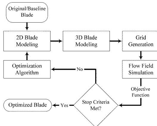
Fig. 9 Flow chart of the automatic optimization loop
