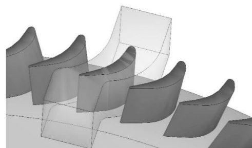
Fig. 5 Stator blade row and control volume for C.F.D. simulations
