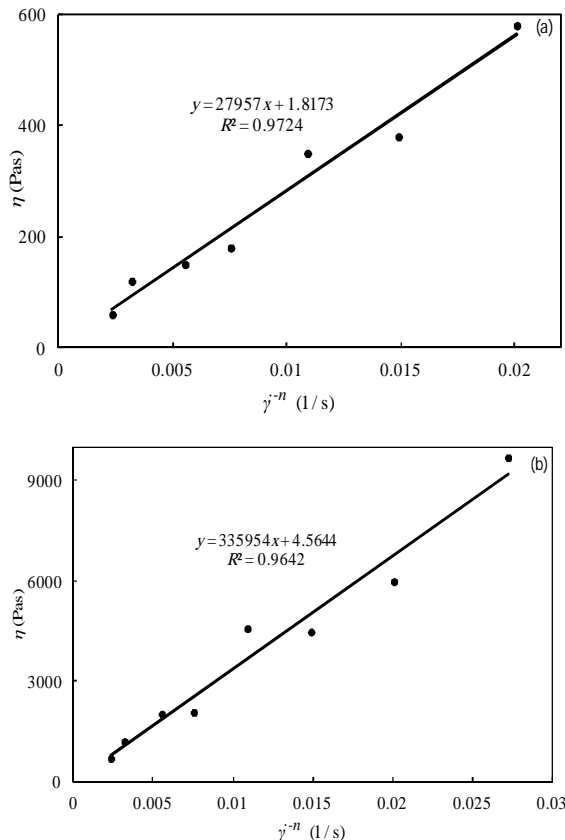
Fig. 10 Calculation of \eta_\infty value based on equation (13) (a) f_s=0.5 , (b) f_s=0.6 شکل 10 محاسبه مقدار \eta_\infty بر اساس معادله (13) (a) f_s=0.5 و (b) f_s=0.6
