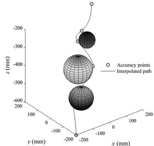
Fig. 14 Optimized trajectory generated by HSA
