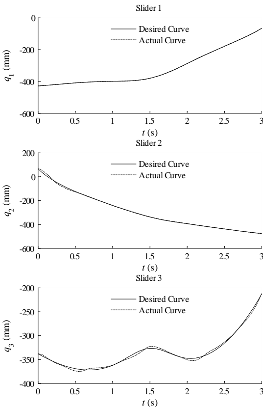
Fig. 11 Sliders motion plots
