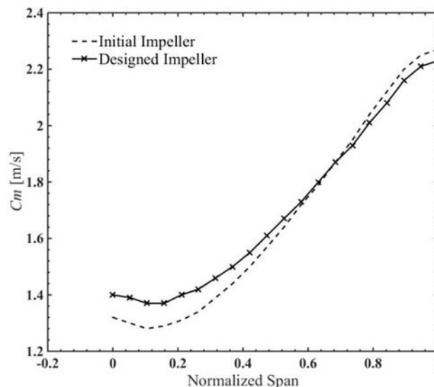
Fig. 16 Meridional Velocity at Leading Edge
