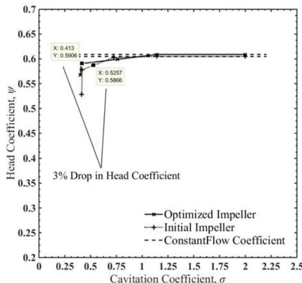
Fig. 17 Cavitation Operation curve for Optimized and current Impeller
