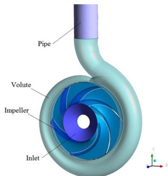
Fig. 5 General View of the Centrifugal Pump Model
