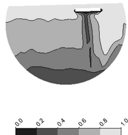
Fig 11. Void Fraction Contour between Collectors
