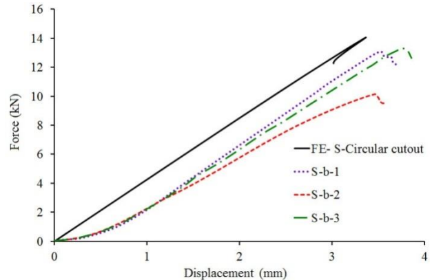
Fig. 14 The force-displacement diagram for unstiffened shell with opening
