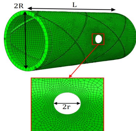
Fig. 7 A finite element model
