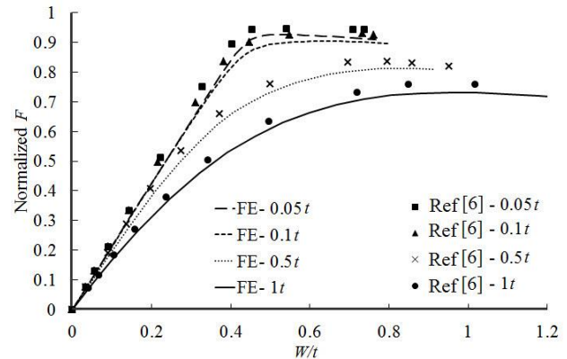
Fig. 8 Validating the finite element model in comparison with the results of Ref [6]
