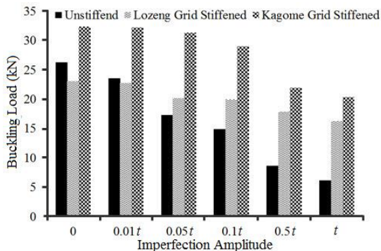
Fig. 17 Buckling load variation of shell with geometric imperfection amplitude
