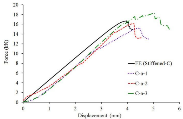
Fig. 11 The force-displacement diagram for stiffened shell type C
