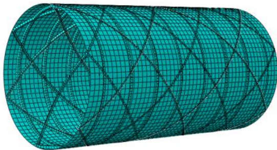
Fig. 16 Stiffened shell with kagome grid
