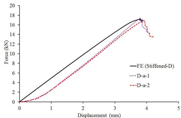
Fig. 12 The force-displacement diagram for stiffened shell type D
