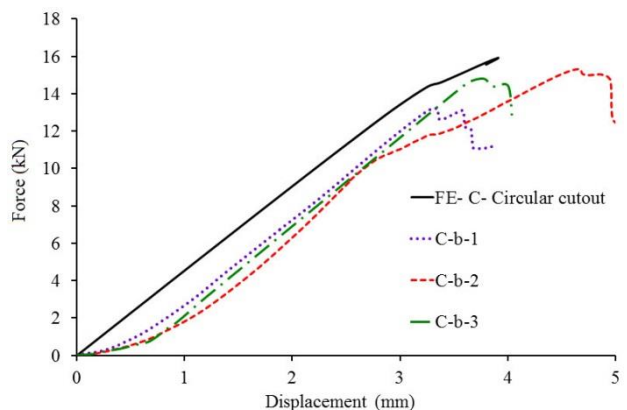
Fig. 15 The force-displacement diagram for stiffened shell type C with opening
