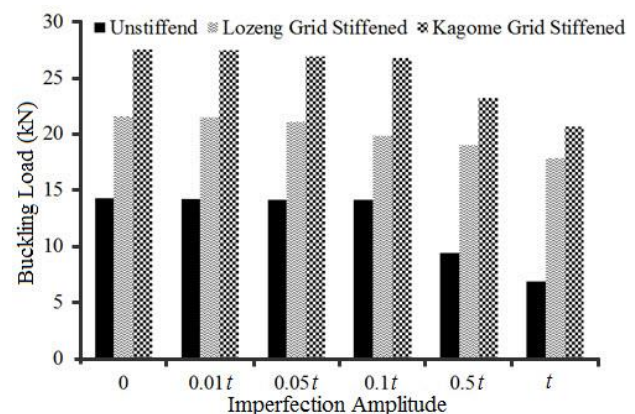
Fig. 18 Buckling load variation of perforated shell with geometric imperfection amplitude
