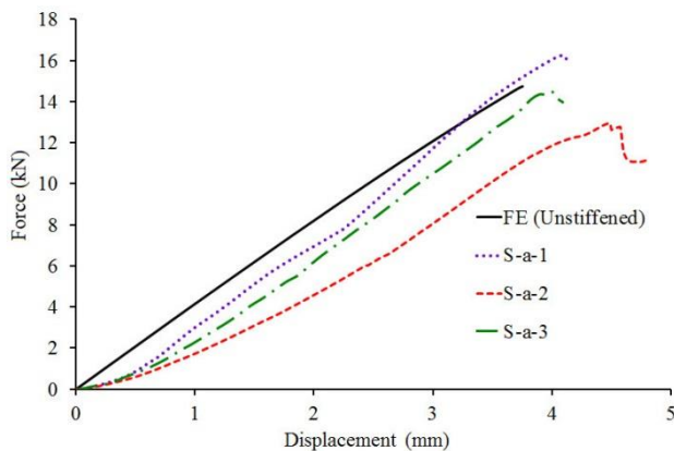
Fig. 10 The force-displacement diagram for unstiffened shell
