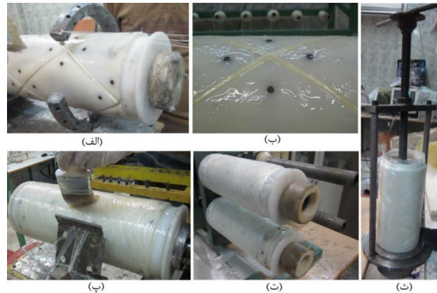
Fig. 2 Manufacturing processes of the grid stiffened shell (a) Manufacturing the ribs, (b) the close view of the grid intersection, (c) winding the outer shell, (d) curing the specimen in room temperature for 8 hours, (e) separating the mold from the specimen
