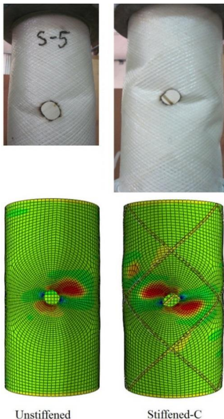
Fig. 13 The buckling shape of shells with a cutout
