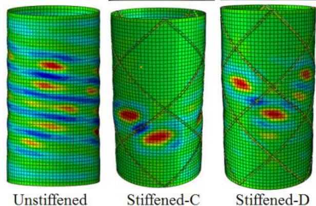
Fig. 9 The buckling shape of shells without cutout
