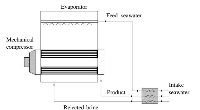
Fig. 1 Schematic of the setup for mechanical vapor compression desalination system and preheater heat exchanger
