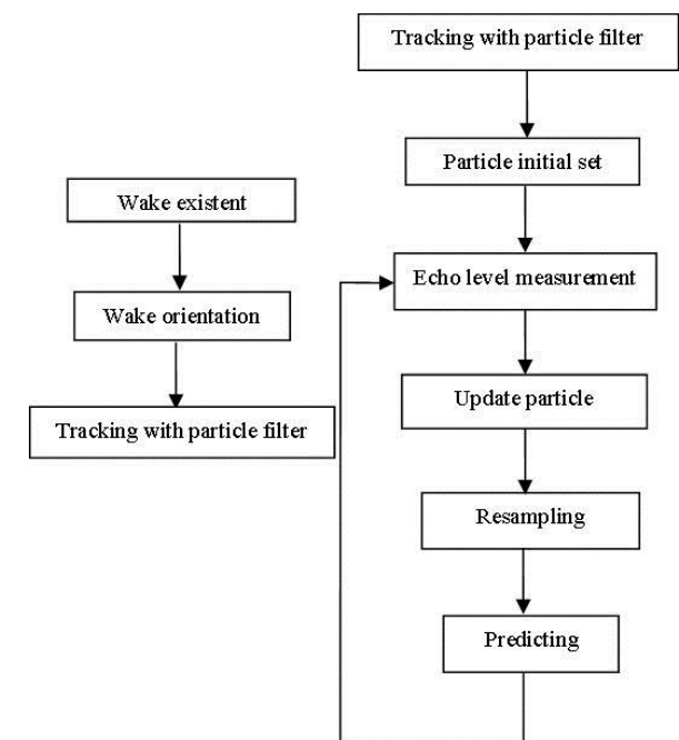
Fig. 4 Tracking algorithm
