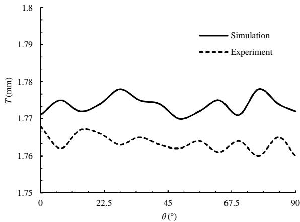
Fig. 14 Thickness of bulged sample along path (a2)
