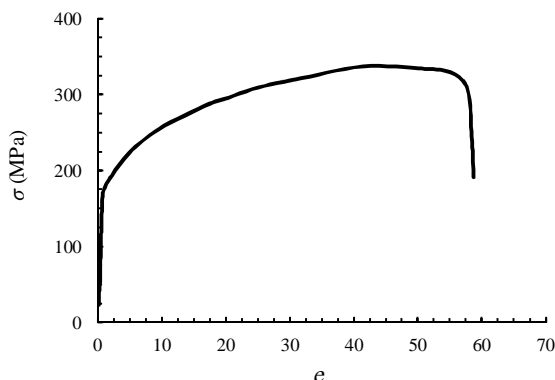
Fig. 3 Engineering Stress-strain curve of brass 70/30-O [15]
