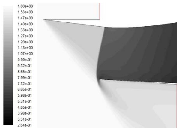
Fig. 3 Mach contour of two dimensional inlet at start condition, M=1.60 , result of solving Euler flow with the accuracy of 10E-05
