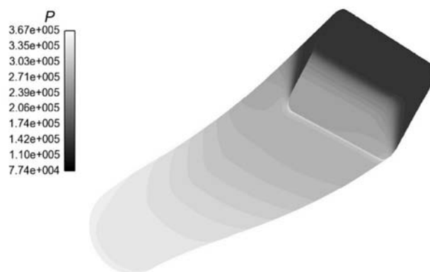
Fig. 19 Pressure distribution on the diffuser (Pa)
