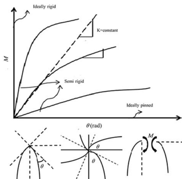
Fig. 5 Semi-rigid connection [24]
