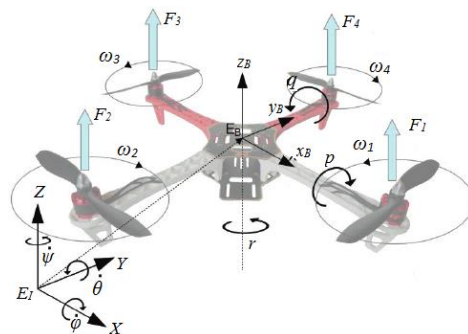
Fig. 2 Quadrotor model with corresponding frames
