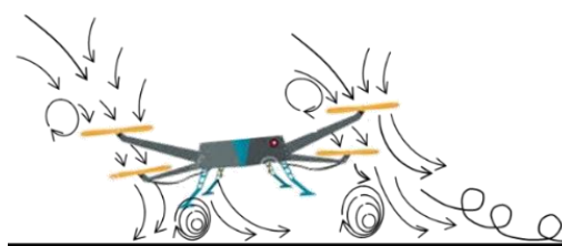
Fig. 1 Formation of Ground Vortex in low speed forward of Quadrotor
