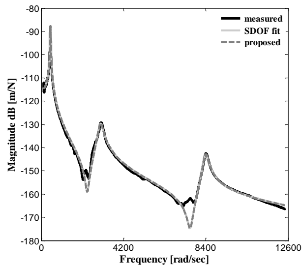
Fig. 6 Comparison of real boring bar point FRF with updated physical model point FRF
