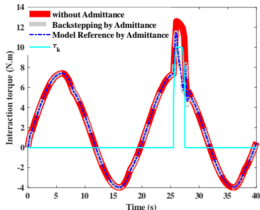
Fig. 9 Interaction torque with admittance control and without it despite involuntary movement of the patient leg
