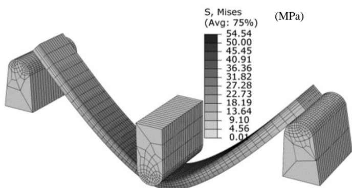
Fig. 5 Finite element modeling of three-point bending test
