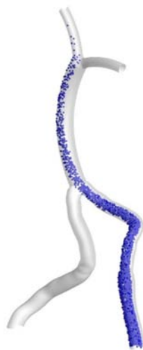
Fig. 21 $4 \mu m$ diameter particles distribution in Vertebrabascular System in the fourth case (particles input from right vertebral)
