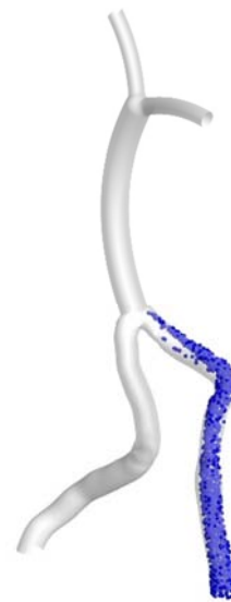
Fig. 18 $4 \mu m$ diameter particles distribution in Vertebrabascular System in the third case
