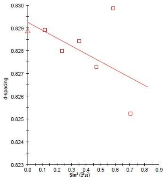
Fig. 7 Linear diagram of d\text{-sin}^2\psi with angle \psi = 0^\circ
