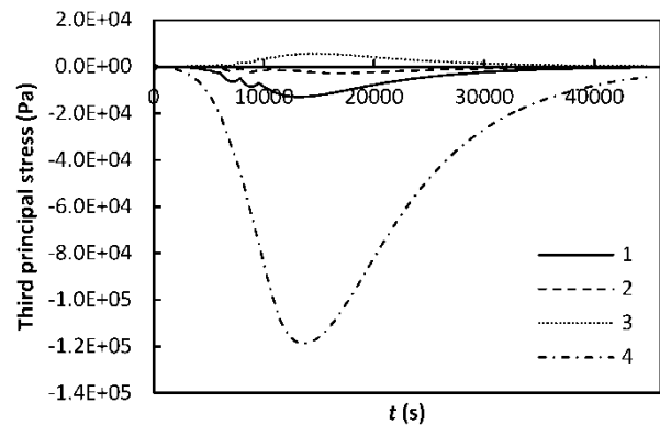
Fig. 16 Third principal stress at four points of the sample
