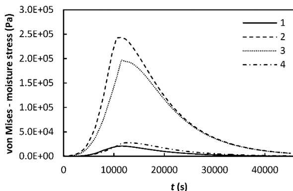
Fig. 17 Von-Mises stress induced by moisture transfer
