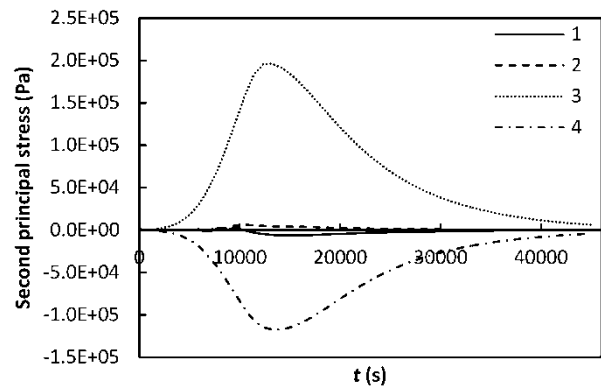
Fig. 15 Second principal stress at four points of the sample
