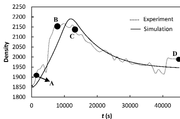
Fig. 8 Total density changes
