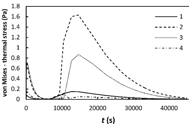
Fig. 18 Von-Mises stress induced by heat transfer
