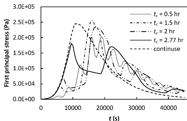
Fig. 23 First principal stress changes in intermittent and continuous drying at point 2
