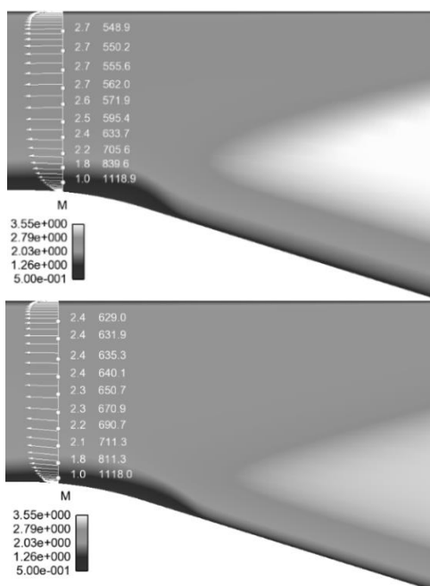
Fig. 13 Effects of attack angle on the internal flow
