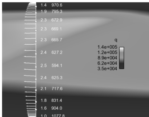
Fig. 19 Dynamic pressure contour and velocity profile before AIP
