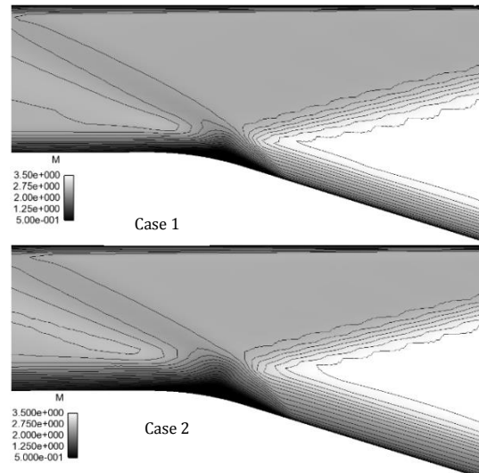
Fig. 10 Close up view of reflexive shock root, A- Case 1, b- Case 2
