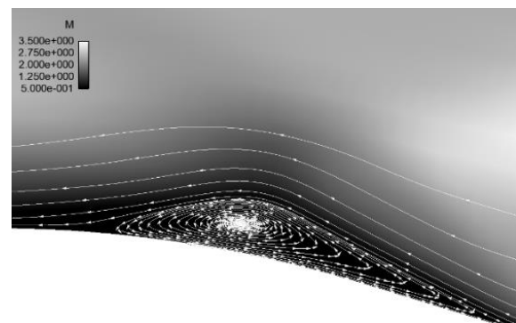
Fig. 11 Streamlines inside the separation region, Case 2
