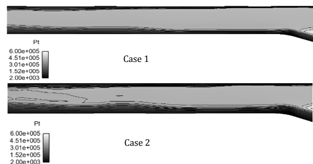
Fig. 12 Duct flow pattern on the plane of symmetry (Pa), a- Case 1, b- Case 2
