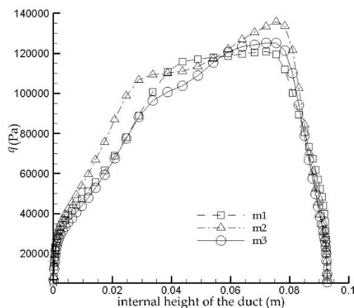
Fig. 20 Dynamic pressure distribution
