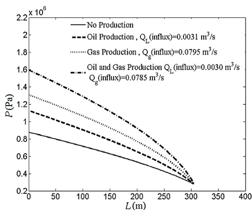
Fig. 19 Effect of oil and gas production on pressure field
