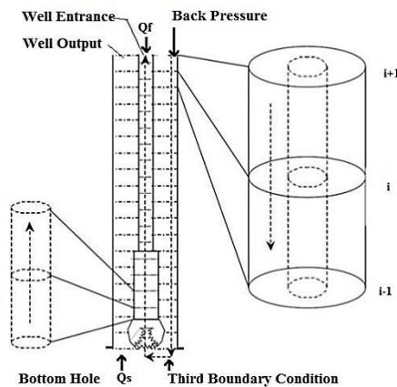
Fig. 3 Computational Grid
