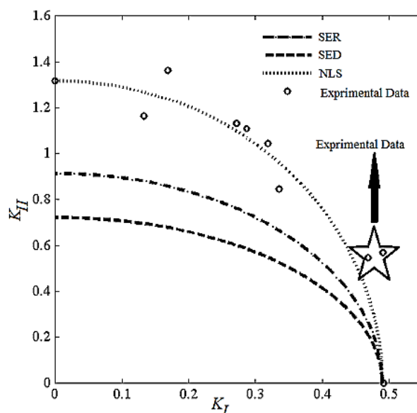
Fig. 4 Fracture limit curves for mixed mode loading of Scot Pine wood in comparison with experimental data[6]
