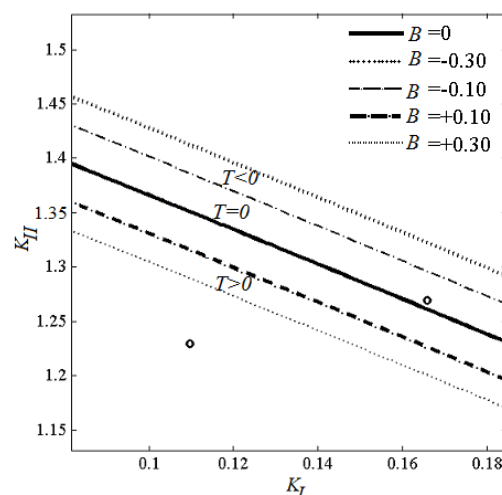
Fig. 15 T-stress effects on fracture limit curves
