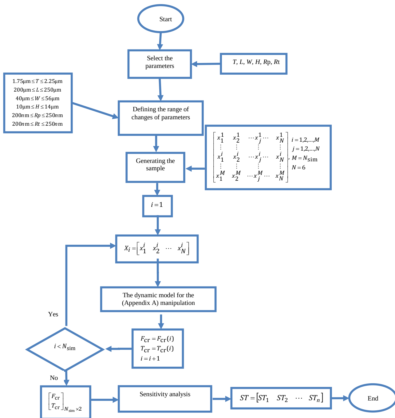
Fig. 2 General algorithm for sensitivity analysis
