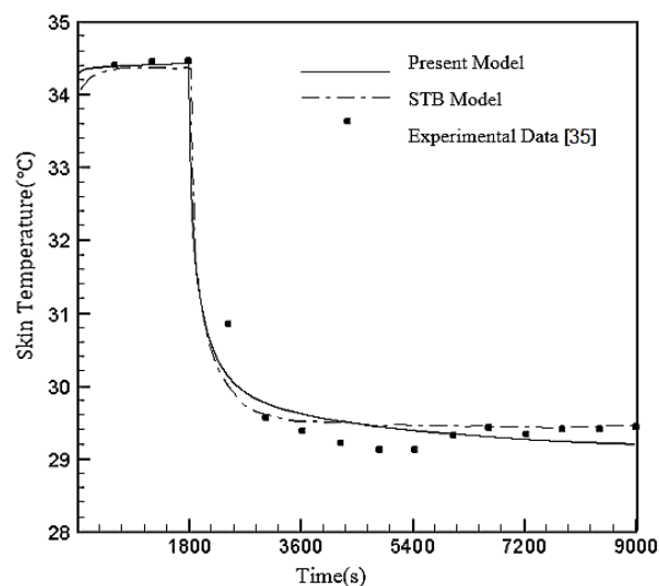
Fig. 3 Comparison of simulated results of new model, measured data [35] and STB model for the skin temperatures
