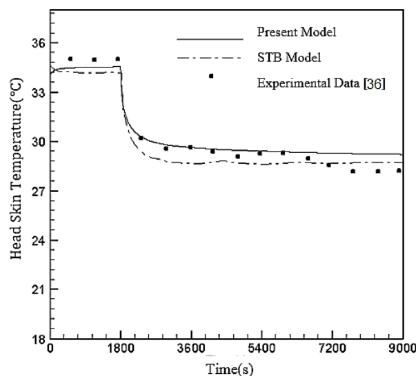
Fig. 4 Comparison of simulated results of new model, measured data [36] and STB model for the skin temperatures
