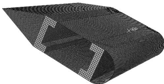
Fig. 8 Modeling the wing sections in finite element software
