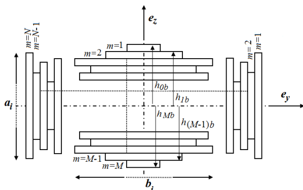
Fig. 2 Public section beam assuming orthotropic symmetric layout
