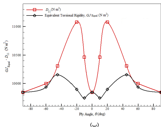
Fig. 9 Variation of stiffness parameters vs. ply angle at the composite wing, a) D_{11} , D_{22} , D_{12} , D_{33} and G_{JEQ} equivalent torsional rigidity, b) Comparing D_{11} , and equivalent torsional rigidity G_{JEQ}
