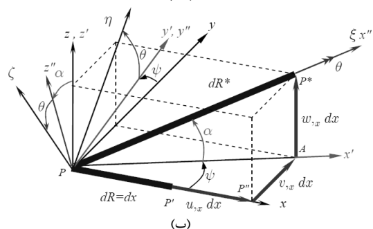
Fig. 4 a) Deformed beam coordinates system b) The displacement and rotation vectors of the element of beam along the main axis [15]
