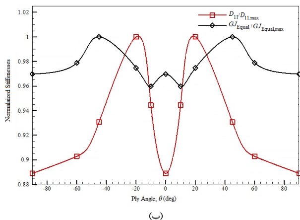
Fig. 10 The effect of angle ply variation on stiffness dimensionless parameters at the composite wing (normalized to the highest value in any direction), a) Normalized D_{11} , D_{22} , D_{12} , D_{33} and GJ_{EQ} equivalent torsional rigidity, b) Comparing Normalized D_{11} and GJ_{EQ}
