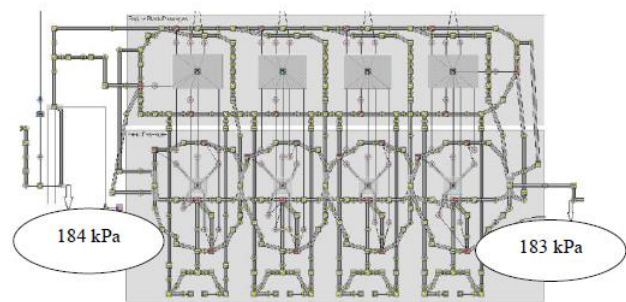
Fig. 4 Coolant pressure in engine channels at the speed of 2000 rpm
