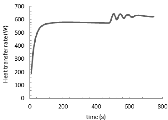
Fig. 11 Heat transfer rate graph from cylinder block wall to fluid cooling of cylinder block No.3
