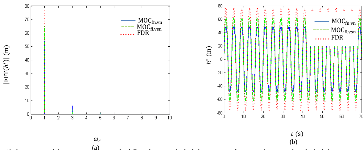
Fig. 13 Comparison of the responses between the full nonlinear method of characteristic, frequency domain and method of characteristic with semi nonlinear valve and linear friction term; (a) output in frequency domain and (b) output in time domain
