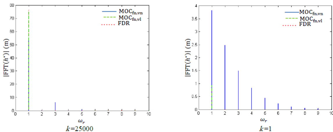
Fig. 4 Comparison of the responses between the full nonlinear method of characteristic, frequency domain and method of characteristic with linear valve and nonlinear friction term
