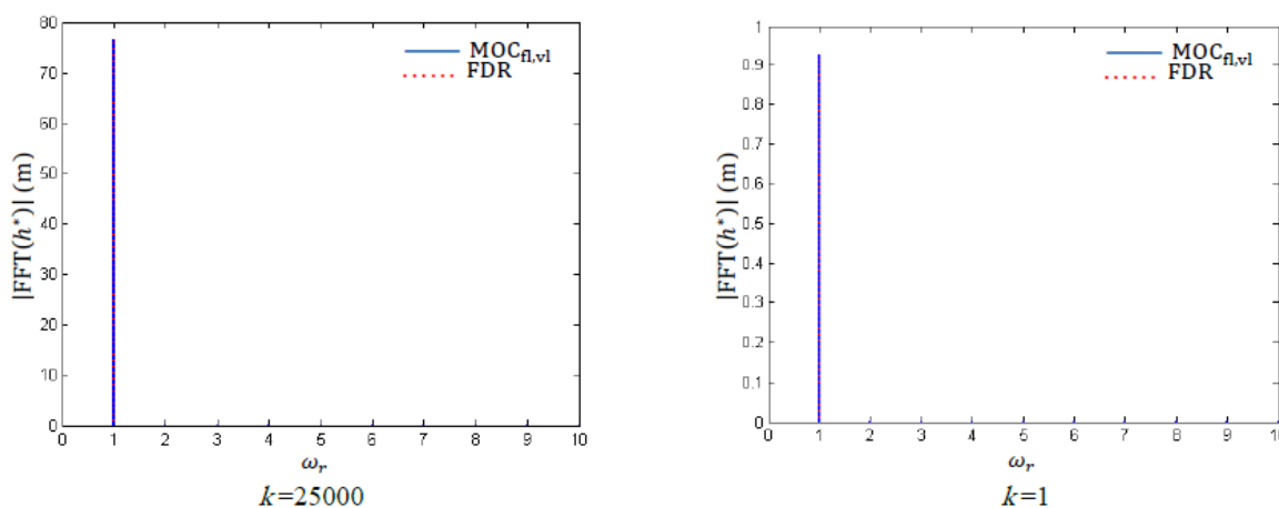
Fig. 3 Comparison of the responses between the full linear method of characteristic and frequency domain
