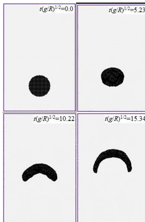
Fig. 1 The rising pattern of an oil plume in a still water tank for different dimensionless times
