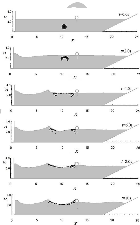
Fig. 12 Simulation the effect of boom with angle 0^\circ on the oil plume dispersion
