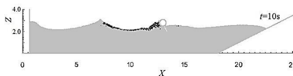
Fig. 14 Simulation of the effect of boom with angle +30^\circ on the oil plume dispersion
