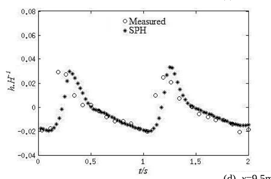
Fig. 8 Comparison between the measured and SPH results for free surface elevations at different positions
