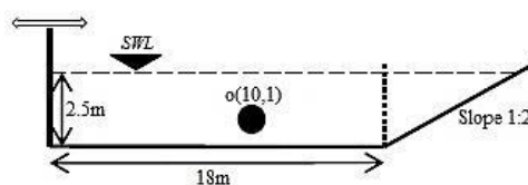
Fig. 9 Initial geometry of the wave flume on the beach
