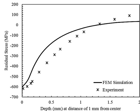
Fig. 4 Radial residual stress field versus depth of the specimen
