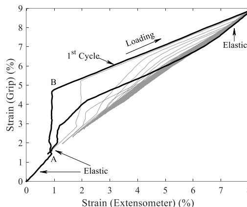
Fig. 8 Evolutions of the global strain versus the local strain during a cyclic tensile test (1 st Cycle)
