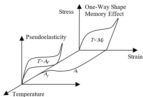
Fig. 2 One-way shape memory effect and pseudoelastic behavior
