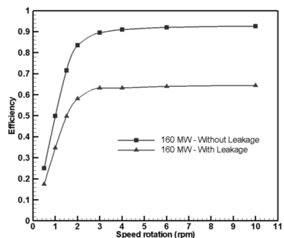
Fig. 14 Effect of rotational speed on the air preheater efficiency in both without and with leakage, 160 MW
