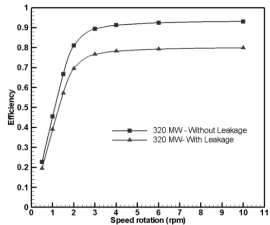
Fig. 12 Effect of rotational speed on the air preheater efficiency in both without and with leakage, 320 MW
