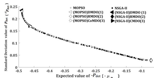
Fig. 6 Pareto optimal solutions for speed uncertainty problem by MOPSO and NSGA-II for (1) DMDO (2) RMDO (3) CMDO
