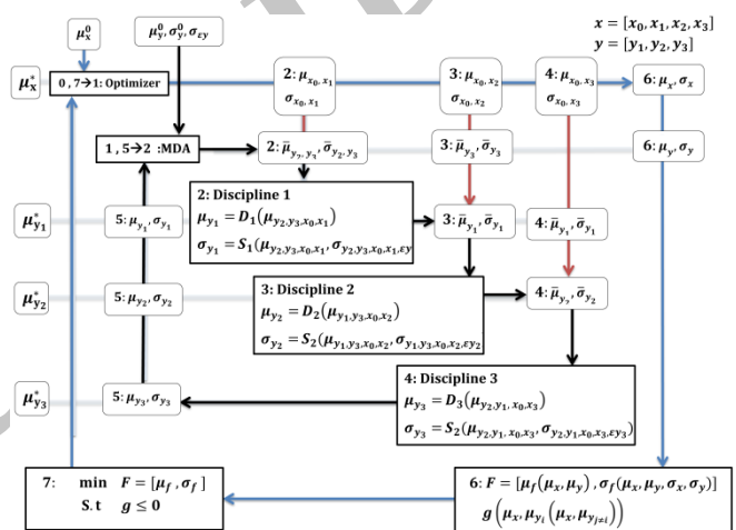
Fig. 1 Structure of UMDF framework for three disciplines
