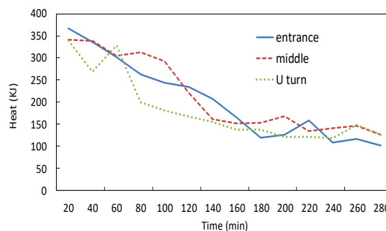
Fig. 11 Total heat transferred from the reservoir every 20 minutes for three different position of the vibrator probe
