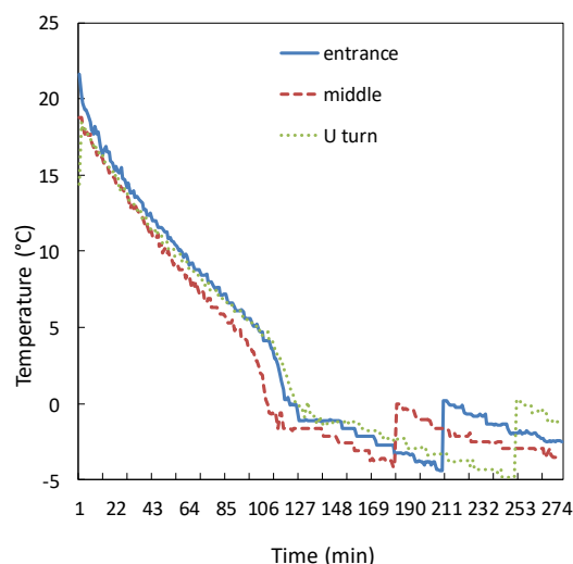
Fig. 9 The temperature recorded by the sensor located on the adjacent coil surface for three different position of the vibrator probe
