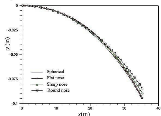
Fig. 25 Trajectory of 5.5 mm-caliber projectiles in vertical x-y plane
