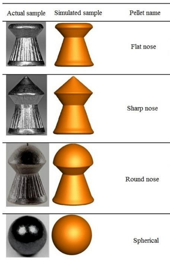
Fig. 1 Comparison of simulated geometries with actual samples
