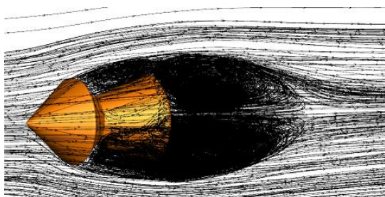
Fig. 19 Instantaneous streamlines past the 4.5 mm-caliber sharp nose projectile
