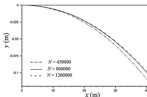
Fig. 7 Comparison of the domed projectile trajectory for different computational grids for M_\infty=0.89 and Re=135000
