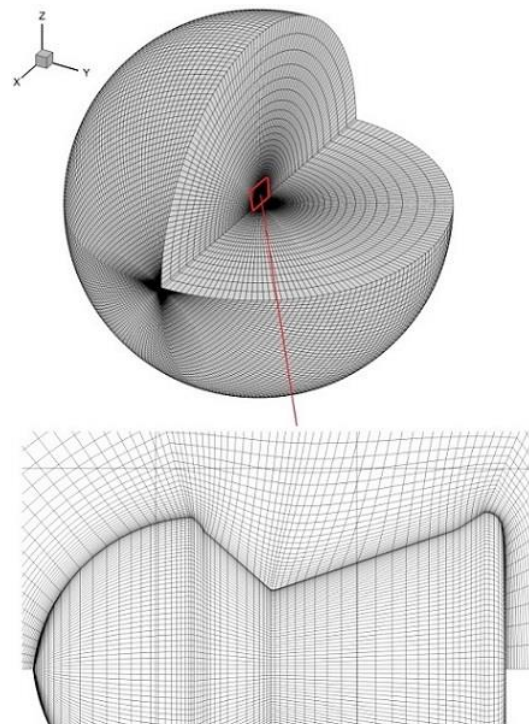
Fig. 5 A grid part used in flow computations
