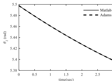
Fig. 3 Comparison of angle of \theta_2 in Adams software & MATLAB software
