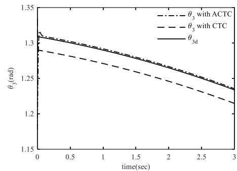
Fig. 28 Comparison of control of angle of \theta_3 by adaptive computed torque control & computed torque control method
