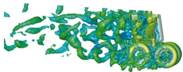
Fig. 1 The location of sound sources in the landing wheels of a volantis
