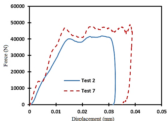
Fig. 19 Comparison of diagram test num. 2&amp;7
