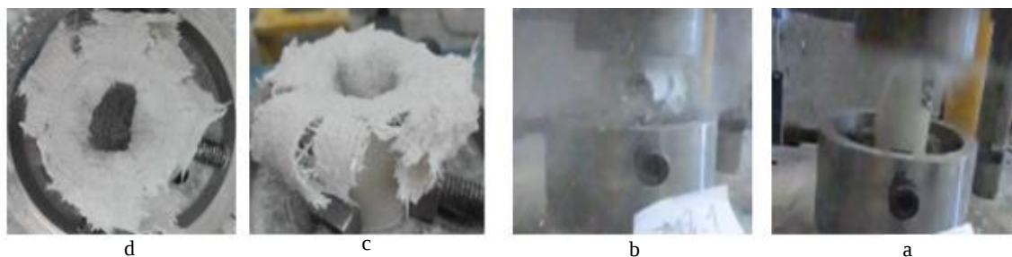
Fig. 26 Failure mode of samples of test 6. a: moment of impact. B: end of impact. c & d :shape of the sample after impact.
