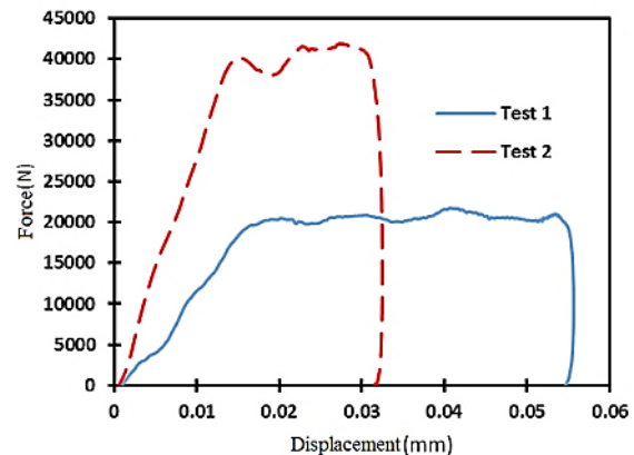
Fig. 13 Comparison of diagram test num. 1&amp;2.
