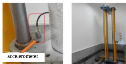
Fig. 9 Drop weight Device and accelerometer connected to it
