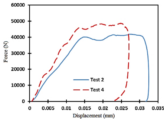
Fig. 15 Comparison of diagram test num. 2&amp;4
