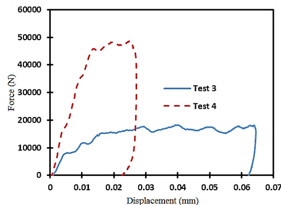
Fig. 16 Comparison of diagram test num. 4&amp;3
