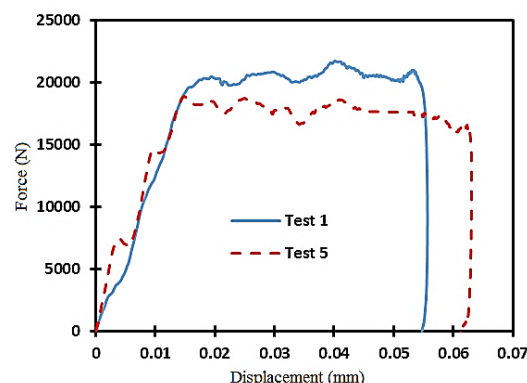
Fig. 17 Comparison of diagram test num. 1&amp;5.
