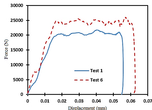
Fig. 18 Comparison of diagram test num. 1&amp;6
