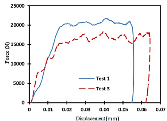
Fig. 14 Comparison of diagram test num. 1&amp;3
