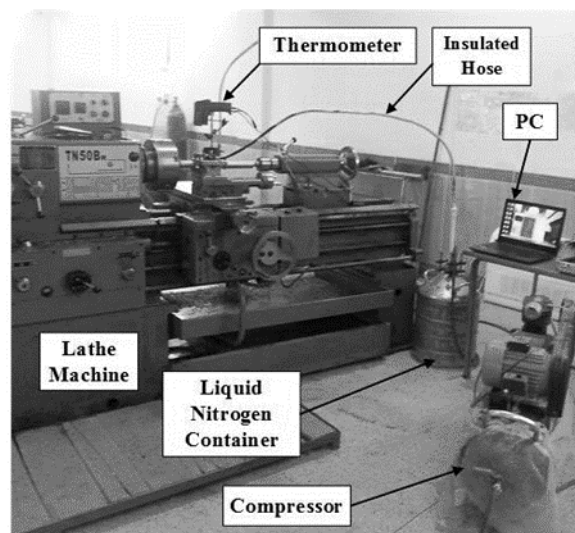
Fig. 4 Lathe machine and the used equipment for cryogenic cooling
