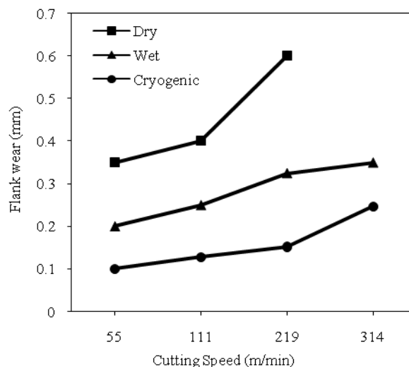
Fig. 11 Flank wear height of tool at different cutting speeds under dry, conventional and cryogenic turning in 0.4 mm/rev feed rate
