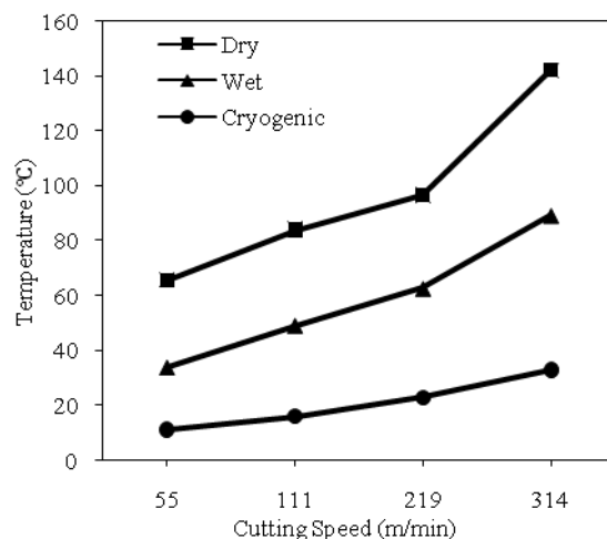
Fig. 8 Comparison of tool temperature in various cutting speeds under dry, conventional and cryogenic turning with 0.4 mm/rev feed rate
