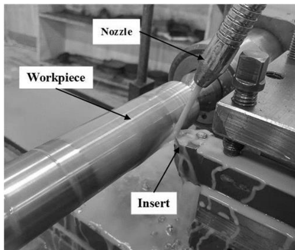
Fig. 5 Wet cooling
