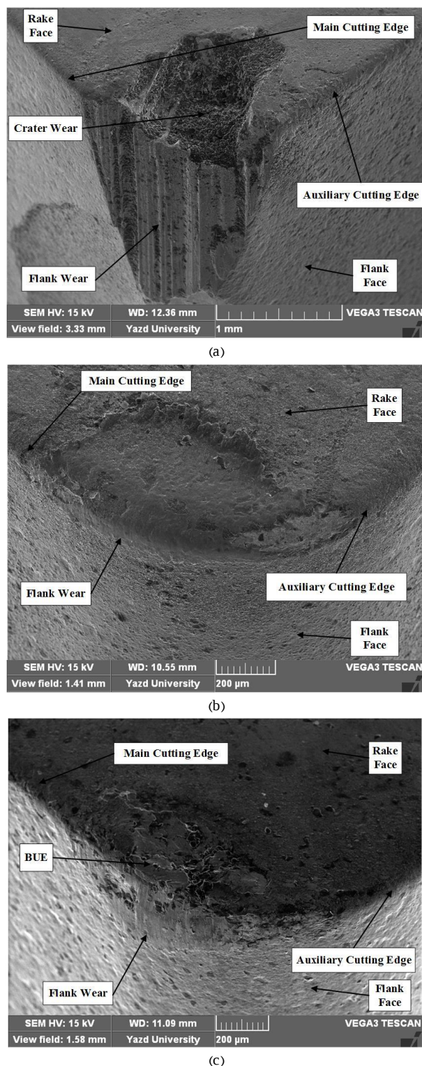
Fig. 13 Tool wear in different states of machining with 0.4 mm/rev feed rate, 314 m/min cutting speed and 1 mm depth of cut, a) dry, b) wet, c) cryogenic
