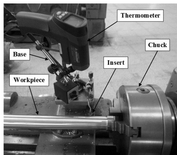
Fig. 3 Measurement of tool temperature by laser thermometer
