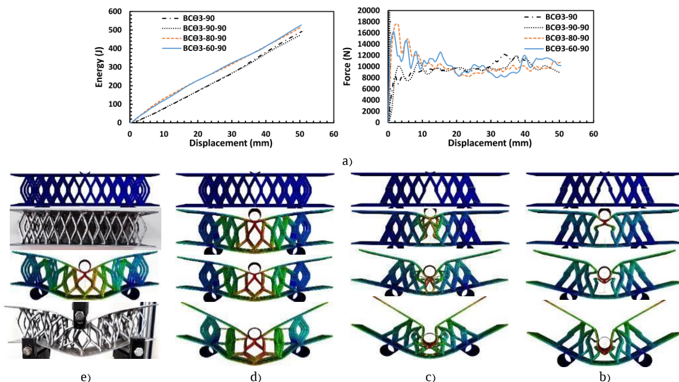
Fig. 16 a) A comparison of force-displacement and energy-displacement curves and collapse of the sandwich structures with lattice core b) BC03-60-90, c) BC03-80-90, d) BC03-90-90, e) BC03-90
