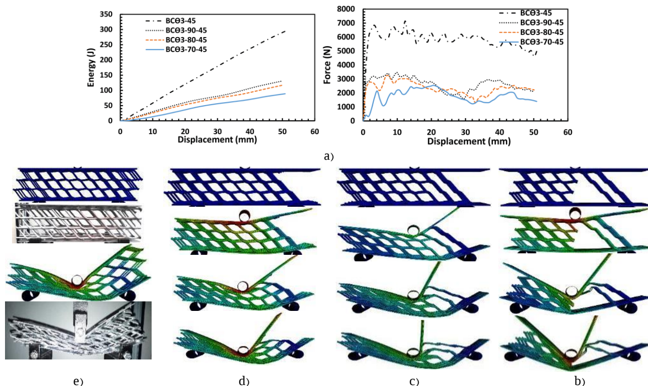
Fig. 15 a) A comparison of force-displacement and energy-displacement curves and collapse of the sandwich structures with lattice core b) BC03-70-45, c) BC03-80-45, d) BC03-90-45, e) BC03-45
