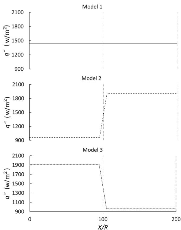
Fig. 6 Three different supplied heat flux models on tube (Model NO.1: Constant, Model NO. 2: Ascending step and Model NO.3: Descending step)
