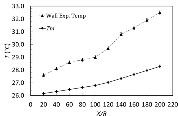
Fig. 9 Experimental bulk and wall temperature distribution for model NO 2.
