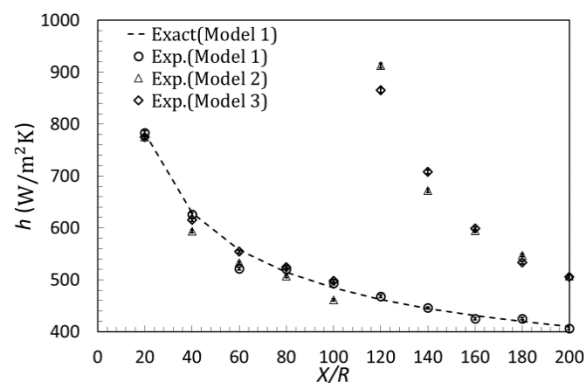
Fig. 7 comparison of Nusselt distribution for three models with Shah equation at Re=1605
